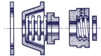
BELLOWS SEAL
